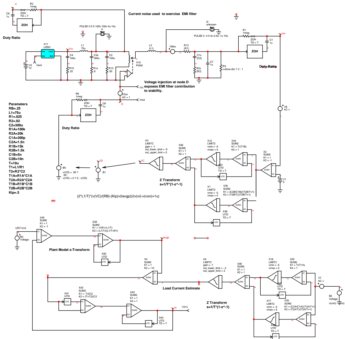
Figure z7 z transform mapped digital control schematic
