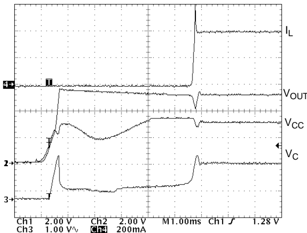
Figure 31. Startup Waveforms of Circuit Shown in the Application Diagram. Load = 400 mA.
