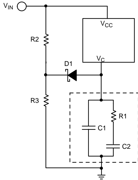
Figure 38. Current Limiting using a Diode Clamp
