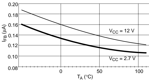
Figure 13. I_{FB} vs. T_A (CS5171/3 only)
