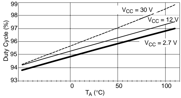
Figure 17. Maximum Duty Cycle vs. T_A
