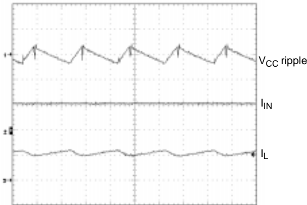
Figure 35. Boost Input Voltage and Current Ripple Waveforms
