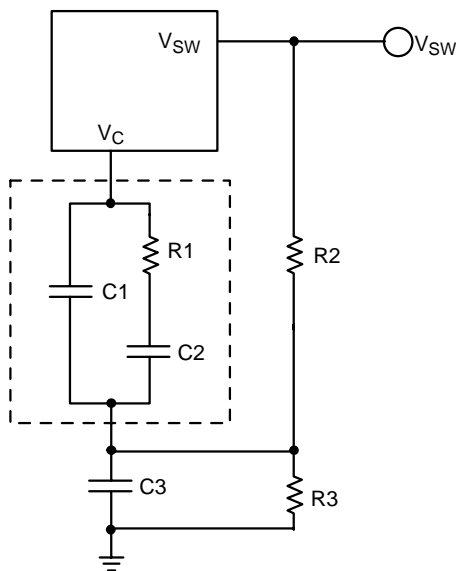
Figure 40. Technique for Increasing Slope Compensation
