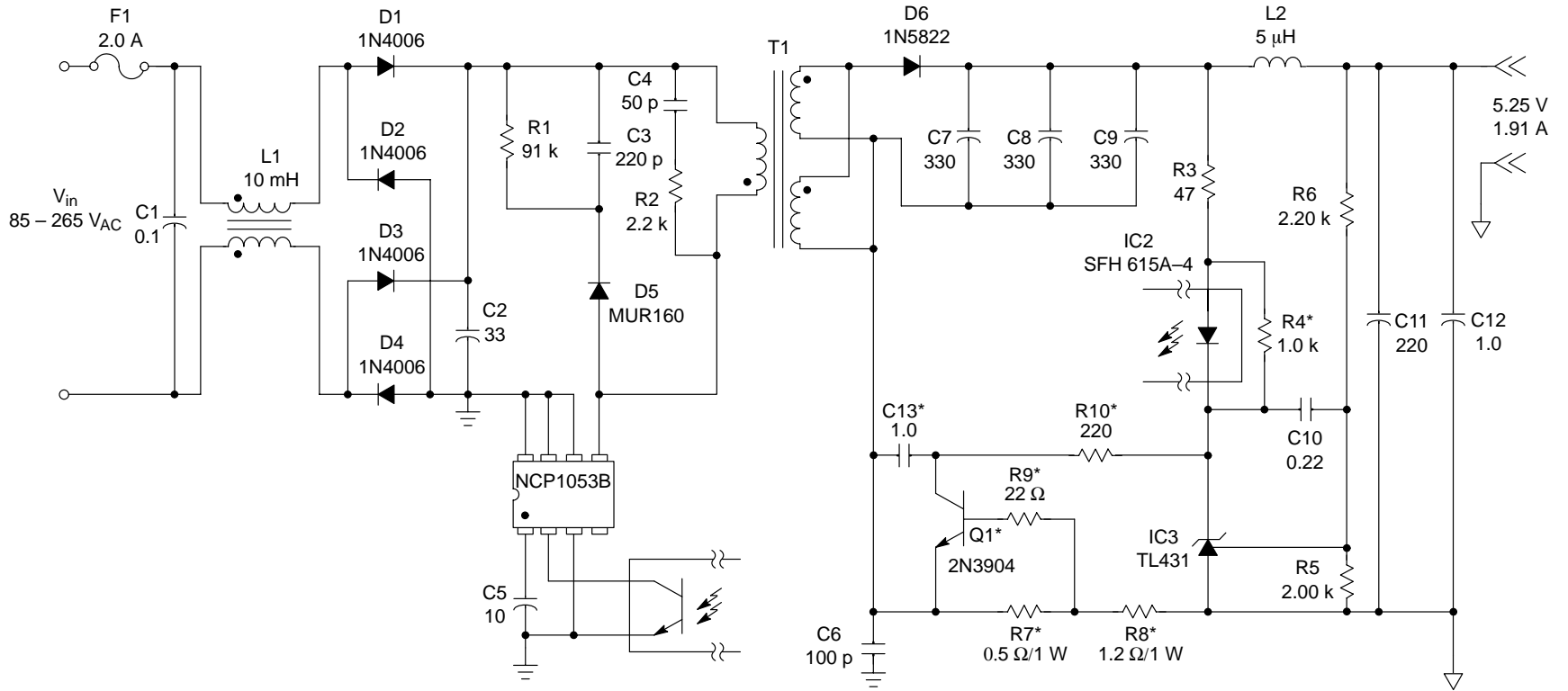
Figure 27. Universal Input 10/5.5 Watt Converter/Charger Application
